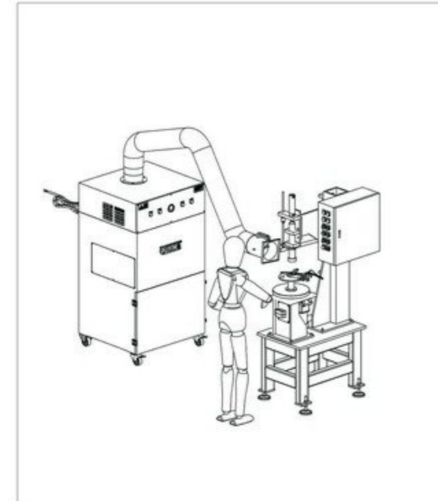
Auto rotation welding machine supported fume extraction
